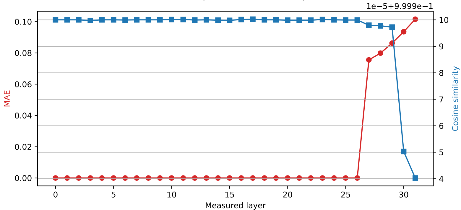
Phi-3-mini-4k-instruct | Quantized layer 26 | float32 → int8
