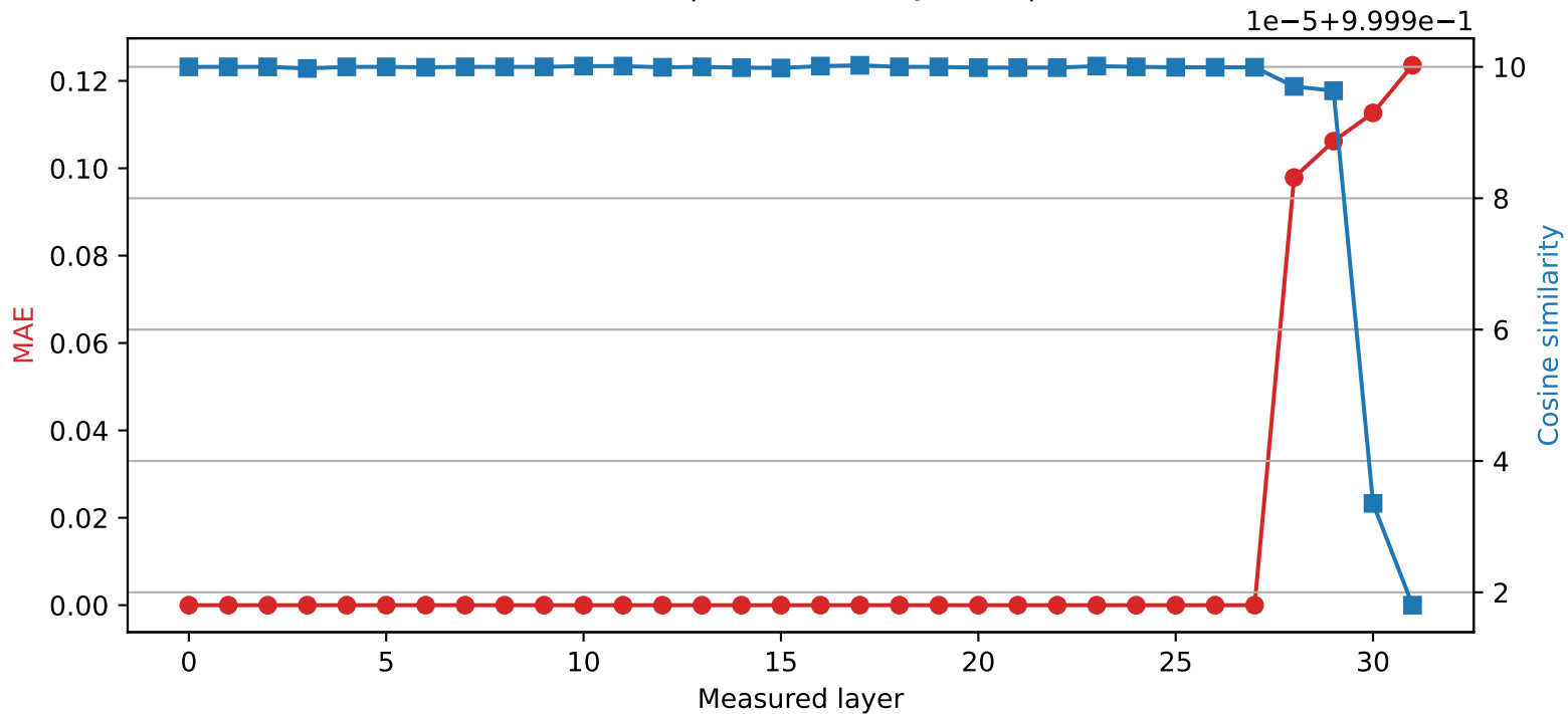
Phi-3-mini-4k-instruct | Quantized layer 27 | float32 \rightarrow int8
