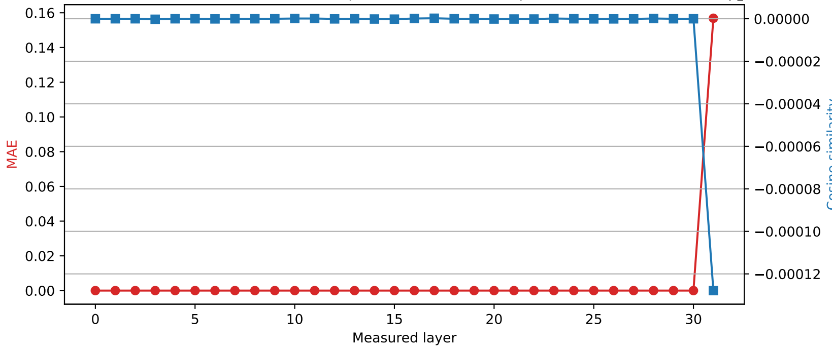
Phi-3-mini-4k-instruct | Quantized layer 30 | float32 \rightarrow int8
