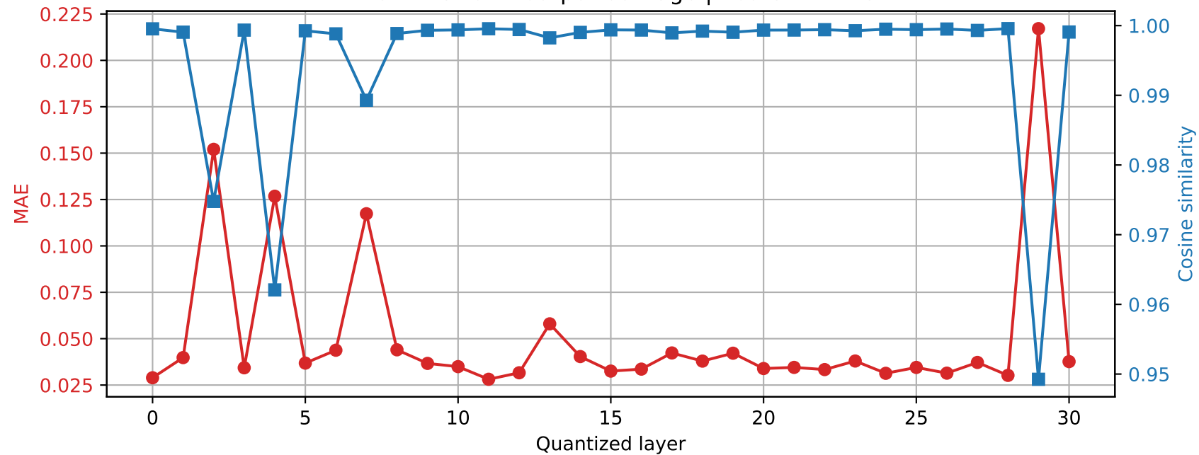
Phi-3-mini-4k-instruct | Prompt 1 Final RMSNorm output damage | float32 \rightarrow int8
