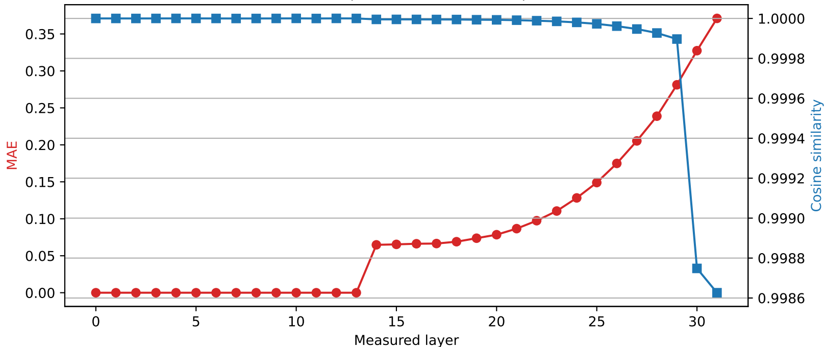
Phi-3-mini-4k-instruct | Quantized layer 13 | float32 \rightarrow int8
