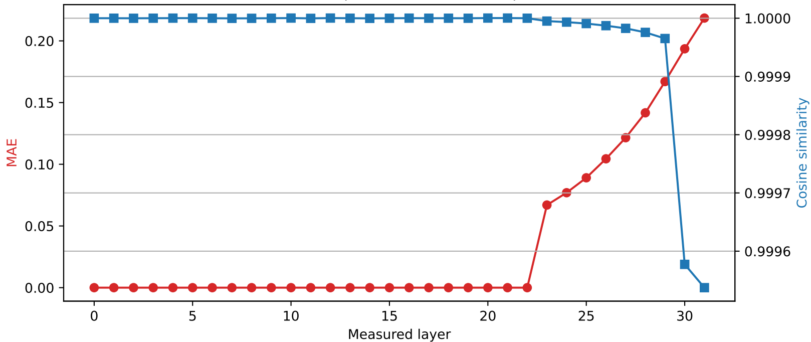
Phi-3-mini-4k-instruct | Quantized layer 22 | float32 \rightarrow int8
