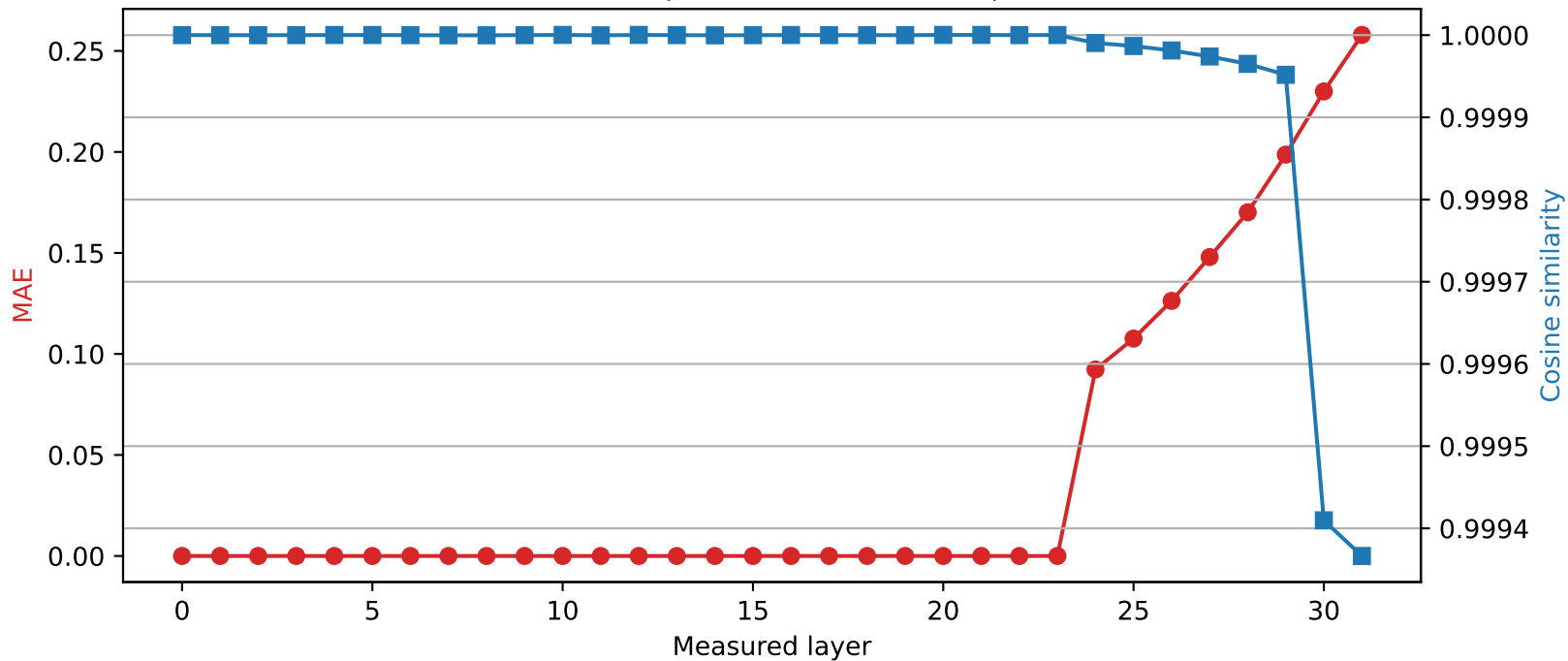
Phi-3-mini-4k-instruct | Quantized layer 23 | float32 \rightarrow int8
