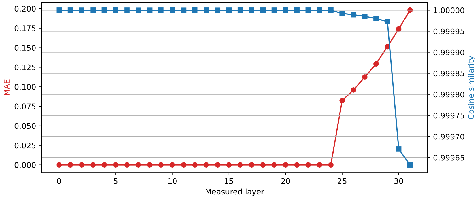
Phi-3-mini-4k-instruct | Quantized layer 24 | float32 \rightarrow int8
