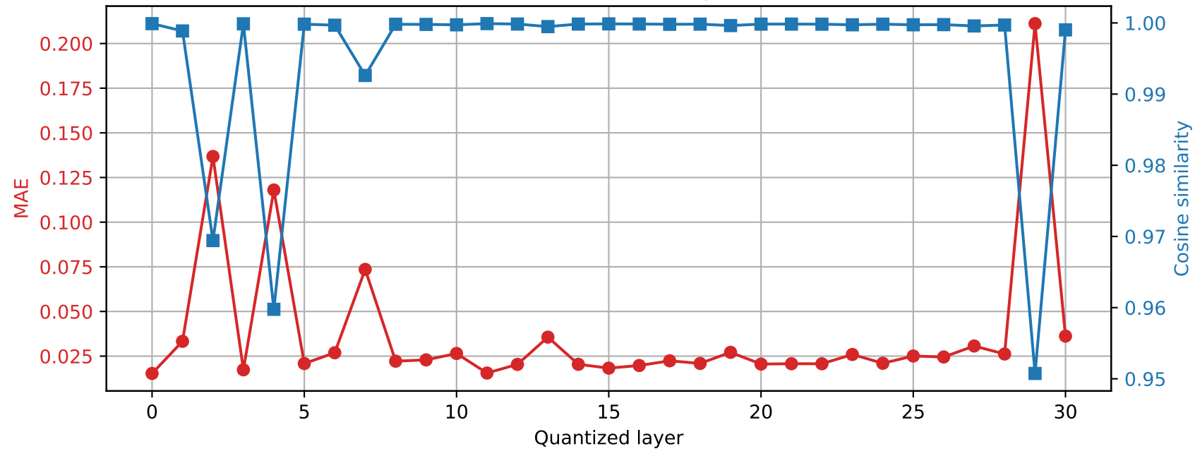
Phi-3-mini-4k-instruct | Prompt 2 Final RMSNorm output damage | float32 \rightarrow int8
