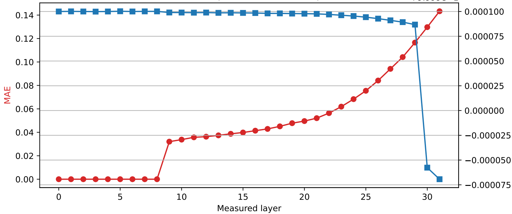
Phi-3-mini-4k-instruct | Quantized layer 8 | float32 \rightarrow int8
