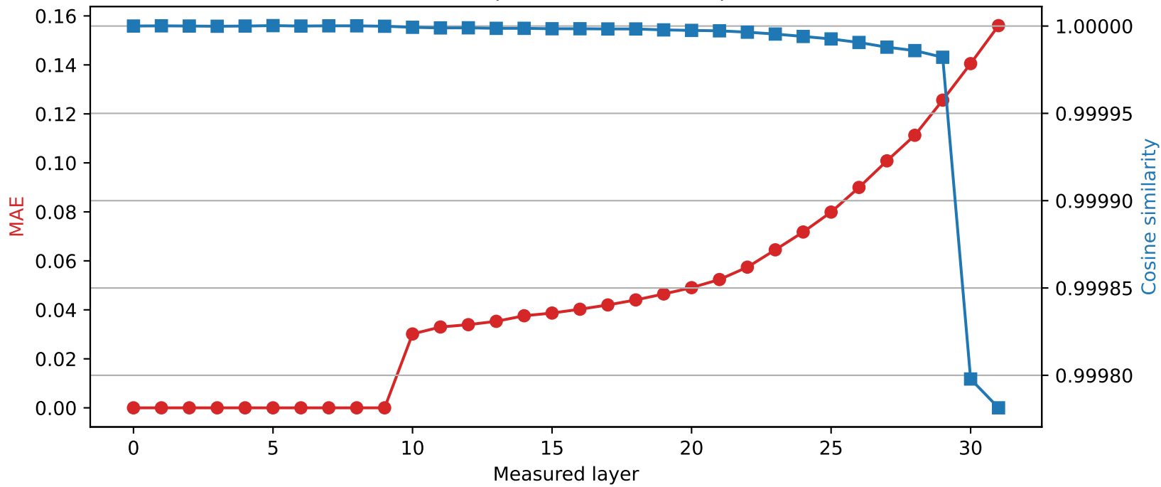
Phi-3-mini-4k-instruct | Quantized layer 9 | float32 \rightarrow int8
