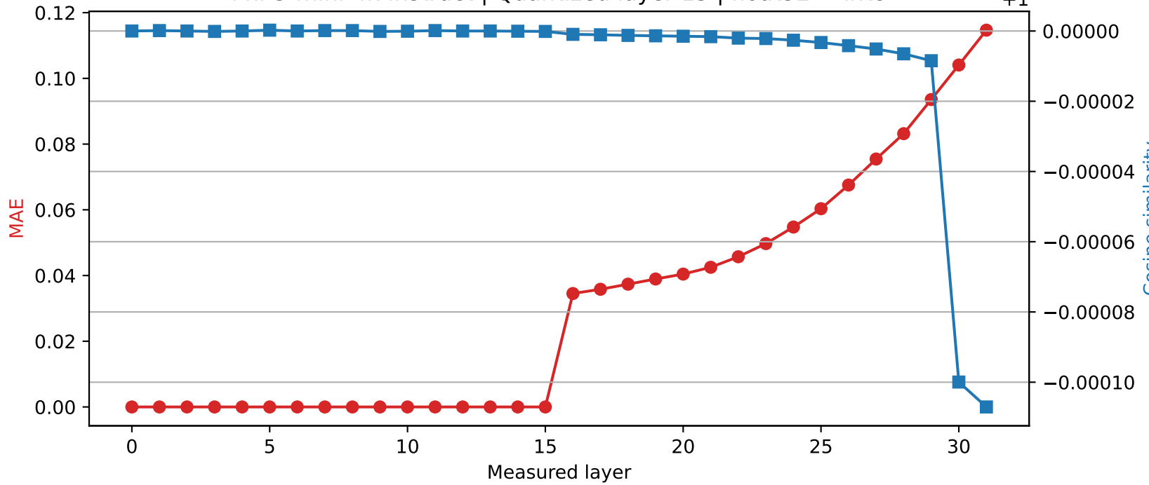
Phi-3-mini-4k-instruct | Quantized layer 15 | float32 \rightarrow int8
