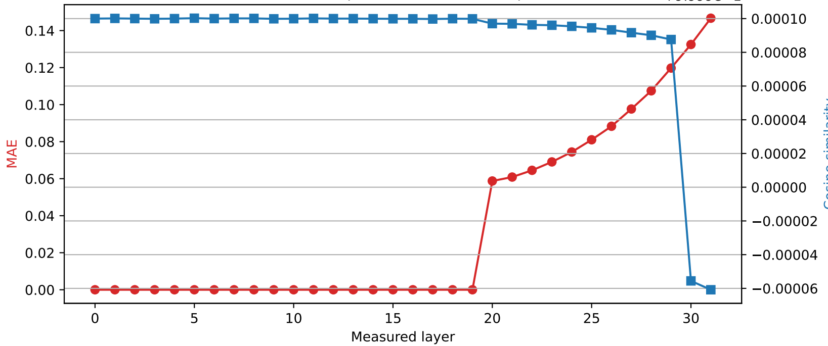
Phi-3-mini-4k-instruct | Quantized layer 19 | float32 \rightarrow int8
