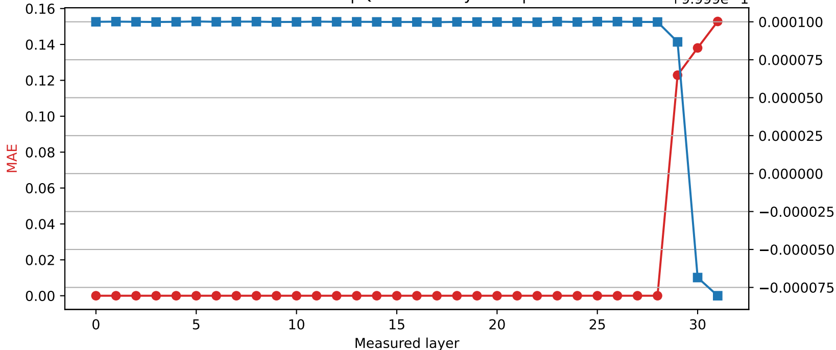
Phi-3-mini-4k-instruct | Quantized layer 28 | float32 \rightarrow int8
