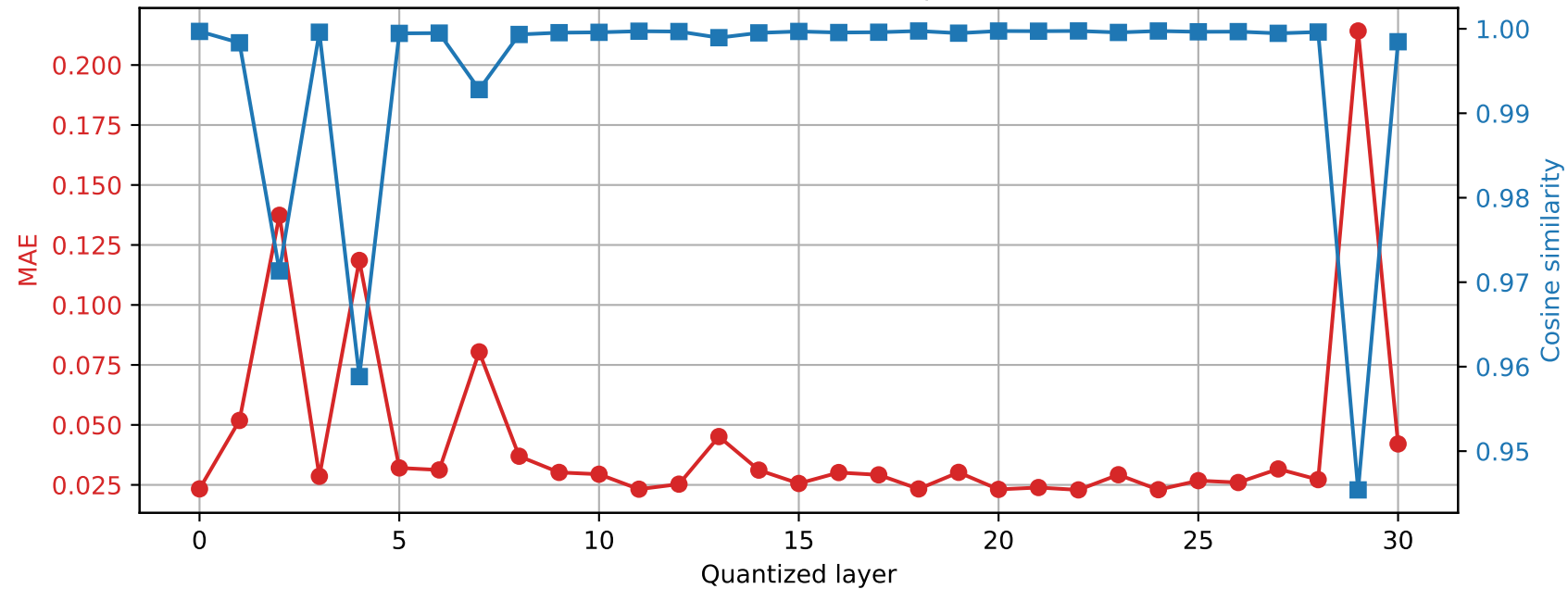
Phi-3-mini-4k-instruct | Prompt 3 Final RMSNorm output damage | float32 \rightarrow int8
