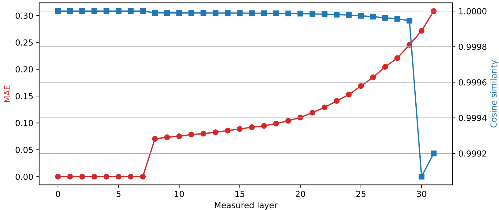
Phi-3-mini-4k-instruct | Quantized layer 7 | float32 \rightarrow int8
