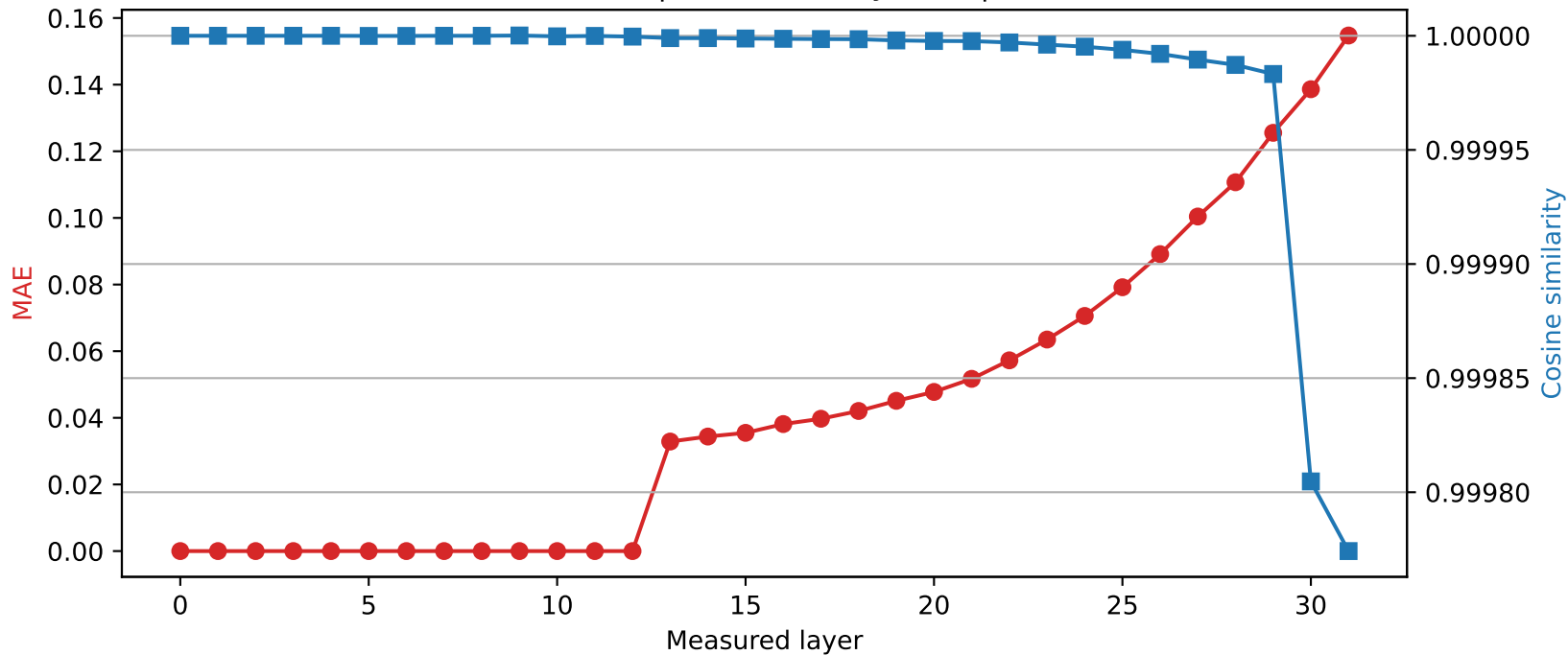
Phi-3-mini-4k-instruct | Quantized layer 12 | float32 \rightarrow int8
