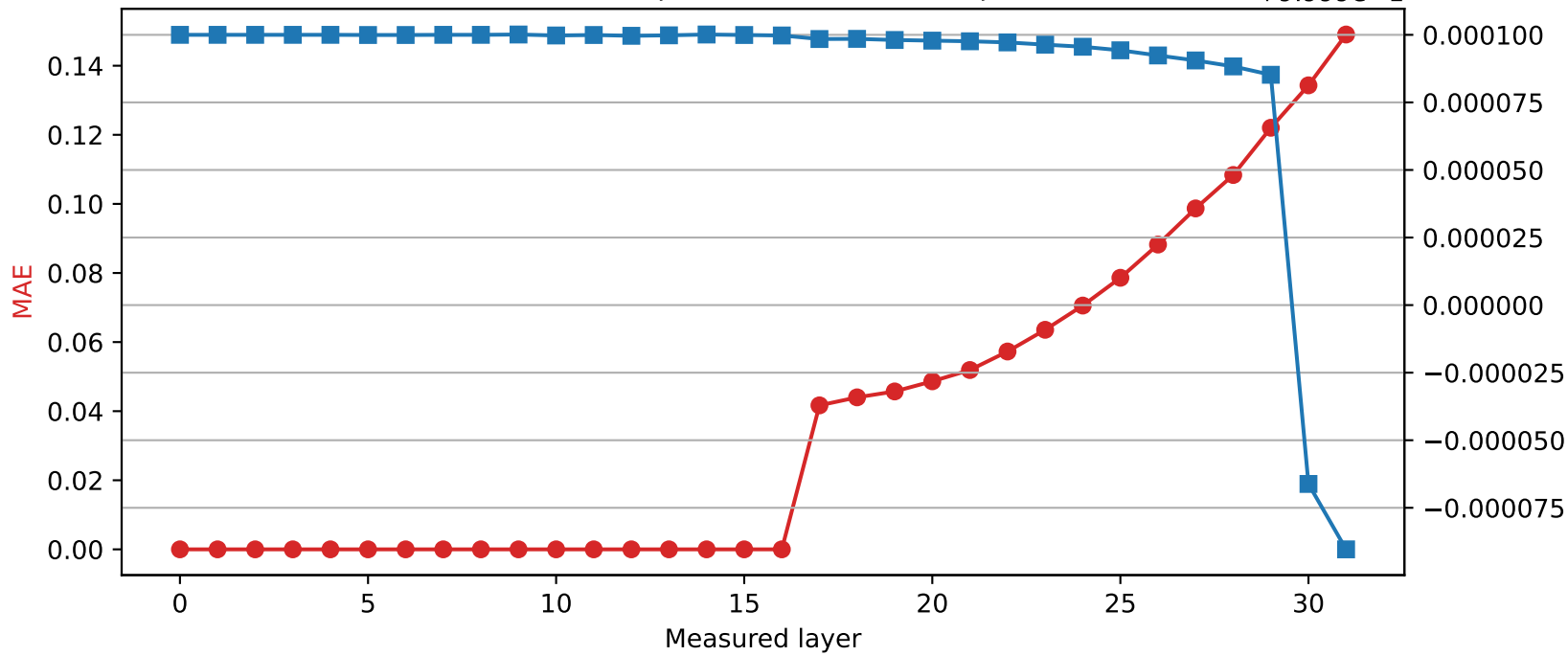
Phi-3-mini-4k-instruct | Quantized layer 16 | float32 → int8
