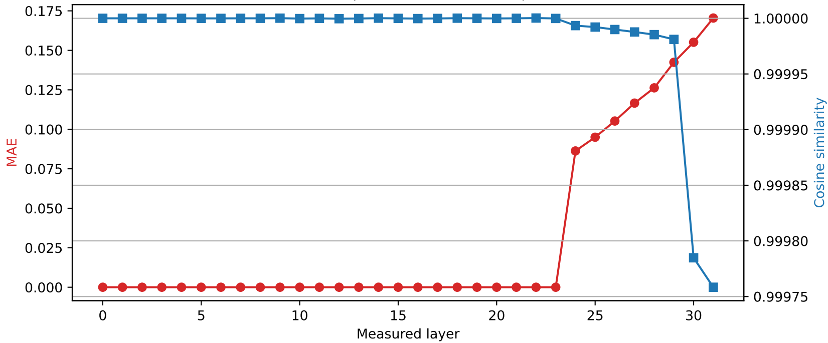
Phi-3-mini-4k-instruct | Quantized layer 23 | float32 \rightarrow int8
