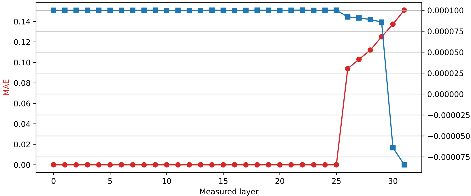
Phi-3-mini-4k-instruct | Quantized layer 25 | float32 \rightarrow int8
