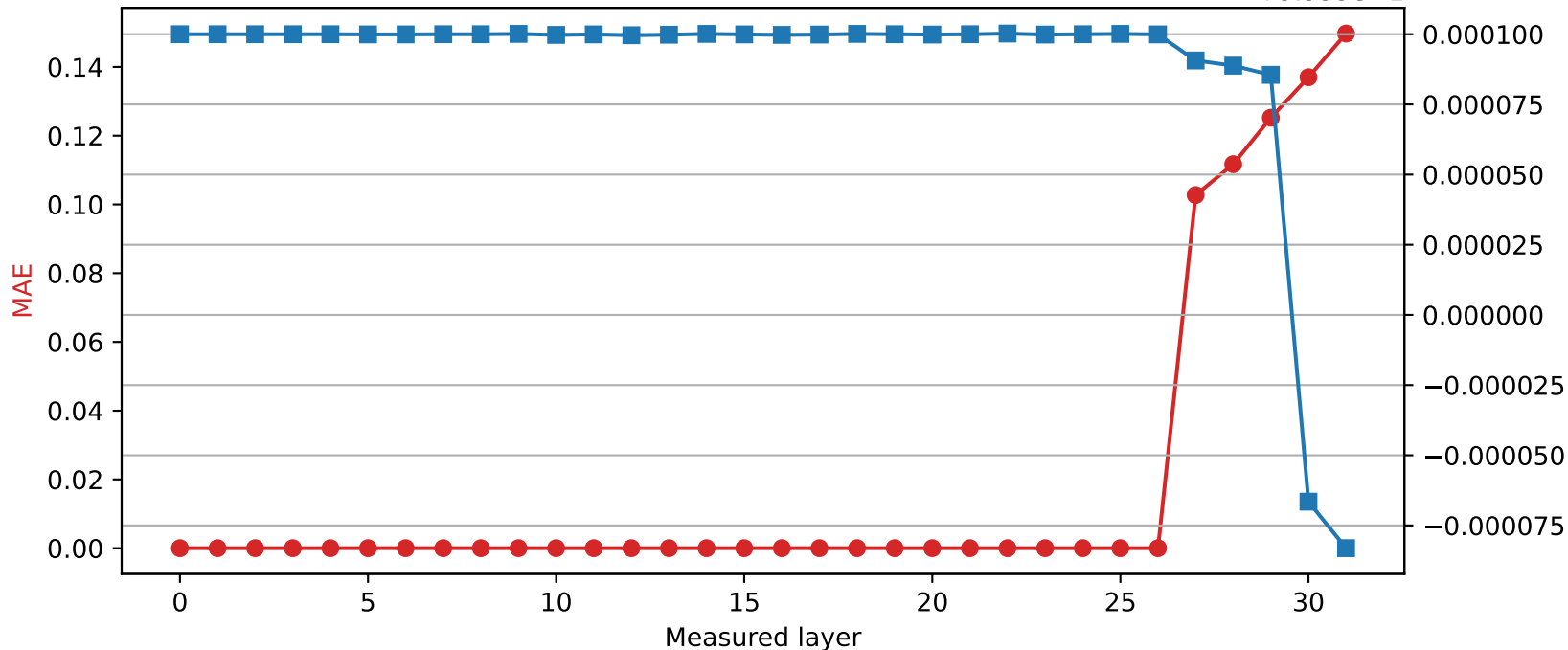
Phi-3-mini-4k-instruct | Quantized layer 26 | float32 → int8
