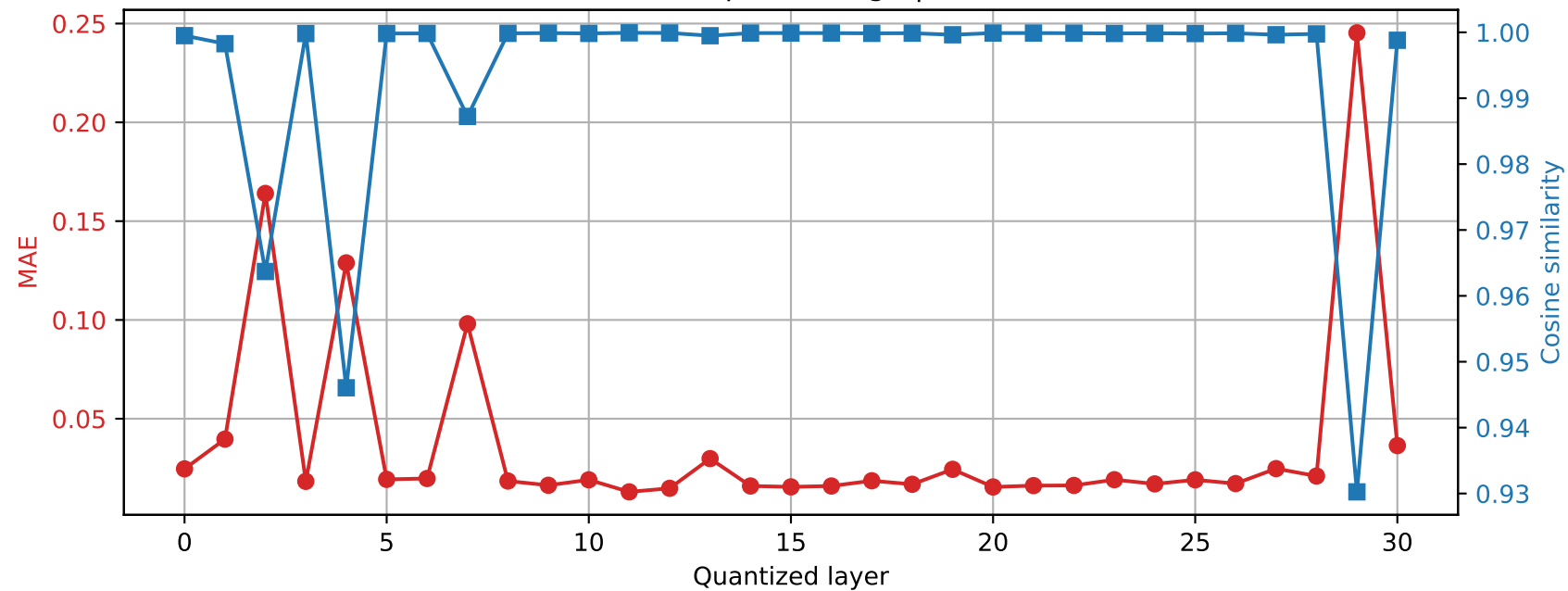
Phi-3-mini-4k-instruct | Prompt 4 Final RMSNorm output damage | float32 \rightarrow int8
