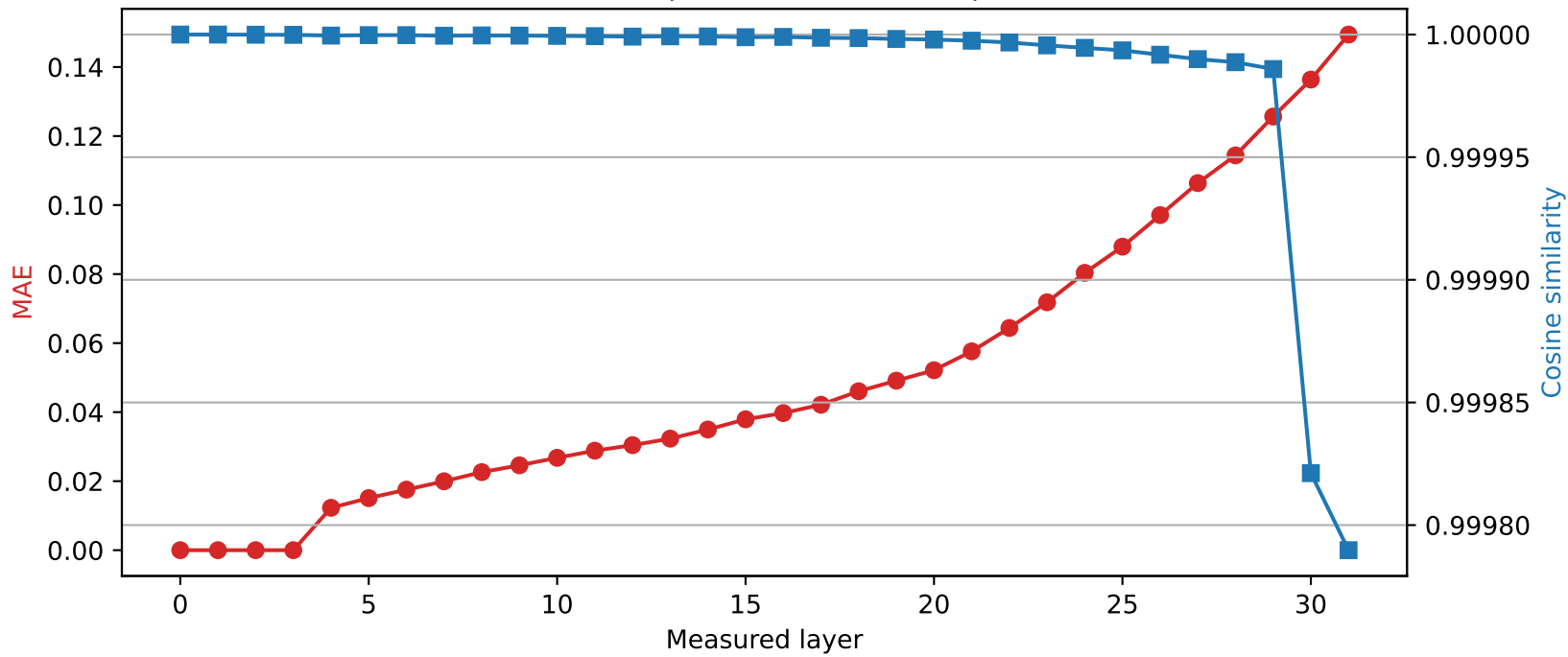
Phi-3-mini-4k-instruct | Quantized layer 3 | float32 \rightarrow int8
