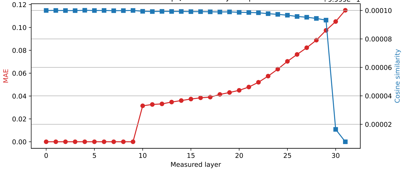
Phi-3-mini-4k-instruct | Quantized layer 9 | float32 \rightarrow int8
