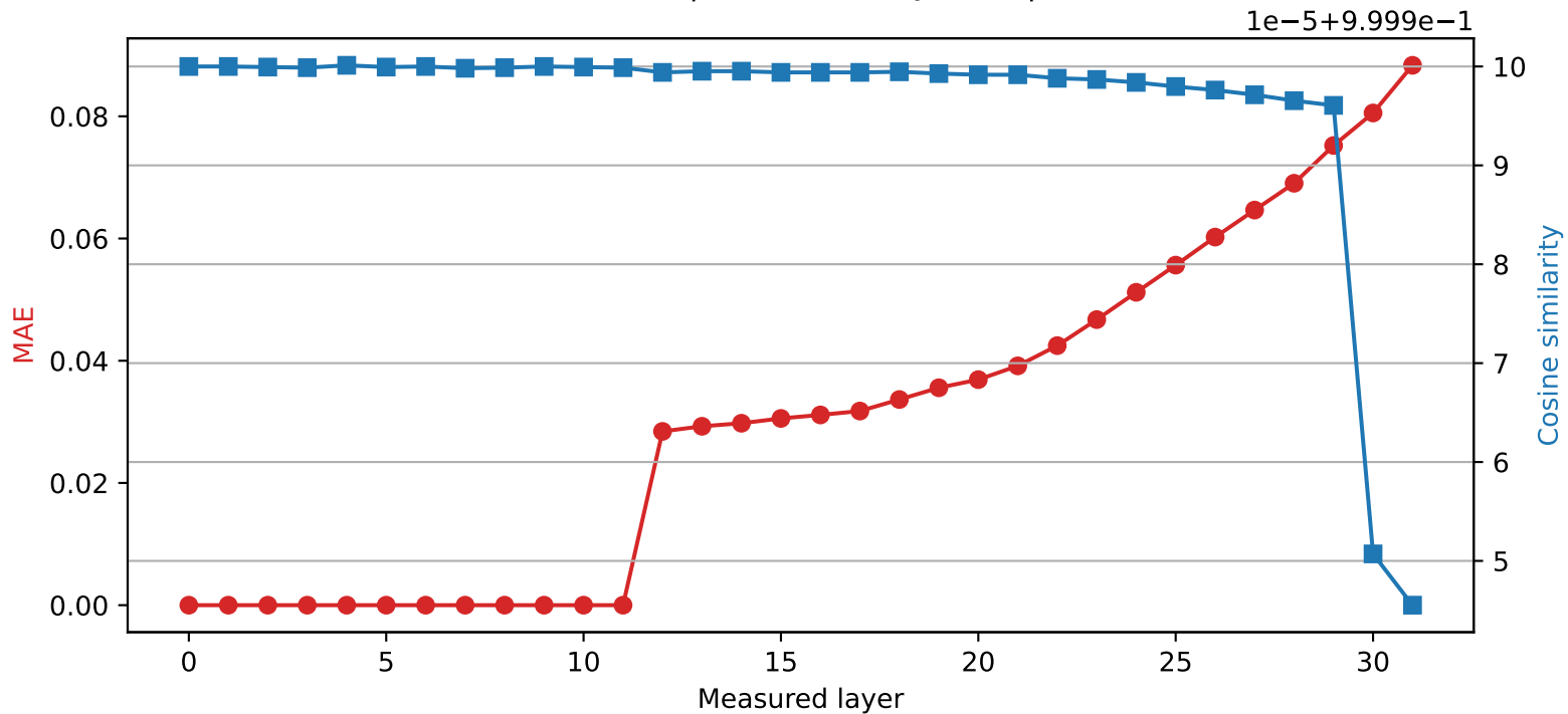
Phi-3-mini-4k-instruct | Quantized layer 11 | float32 → int8
