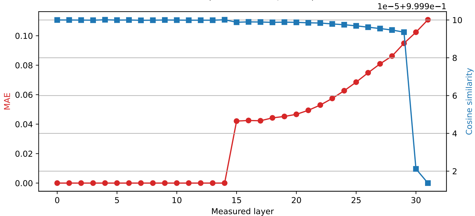
Phi-3-mini-4k-instruct | Quantized layer 14 | float32 \rightarrow int8
