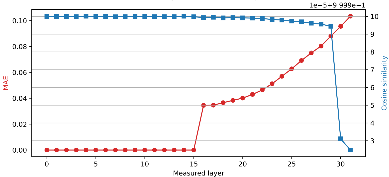
Phi-3-mini-4k-instruct | Quantized layer 15 | float32 \rightarrow int8
