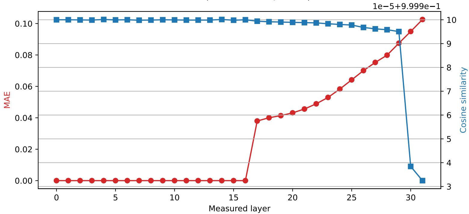
Phi-3-mini-4k-instruct | Quantized layer 16 | float32 \rightarrow int8
