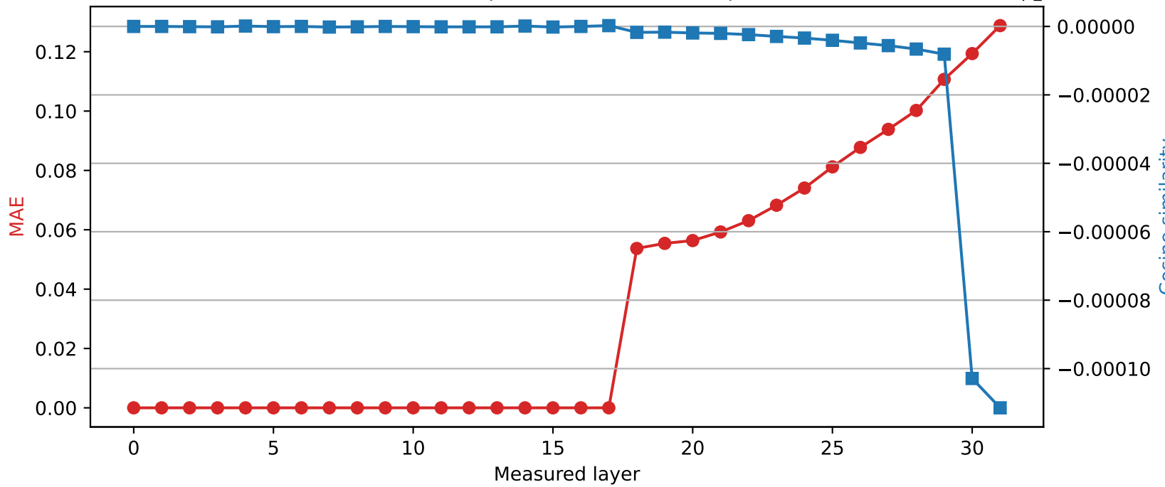
Phi-3-mini-4k-instruct | Quantized layer 17 | float32 \rightarrow int8
