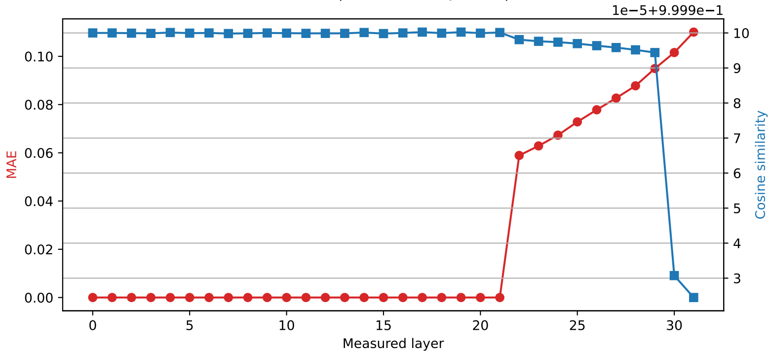
Phi-3-mini-4k-instruct | Quantized layer 21 | float32 \rightarrow int8
