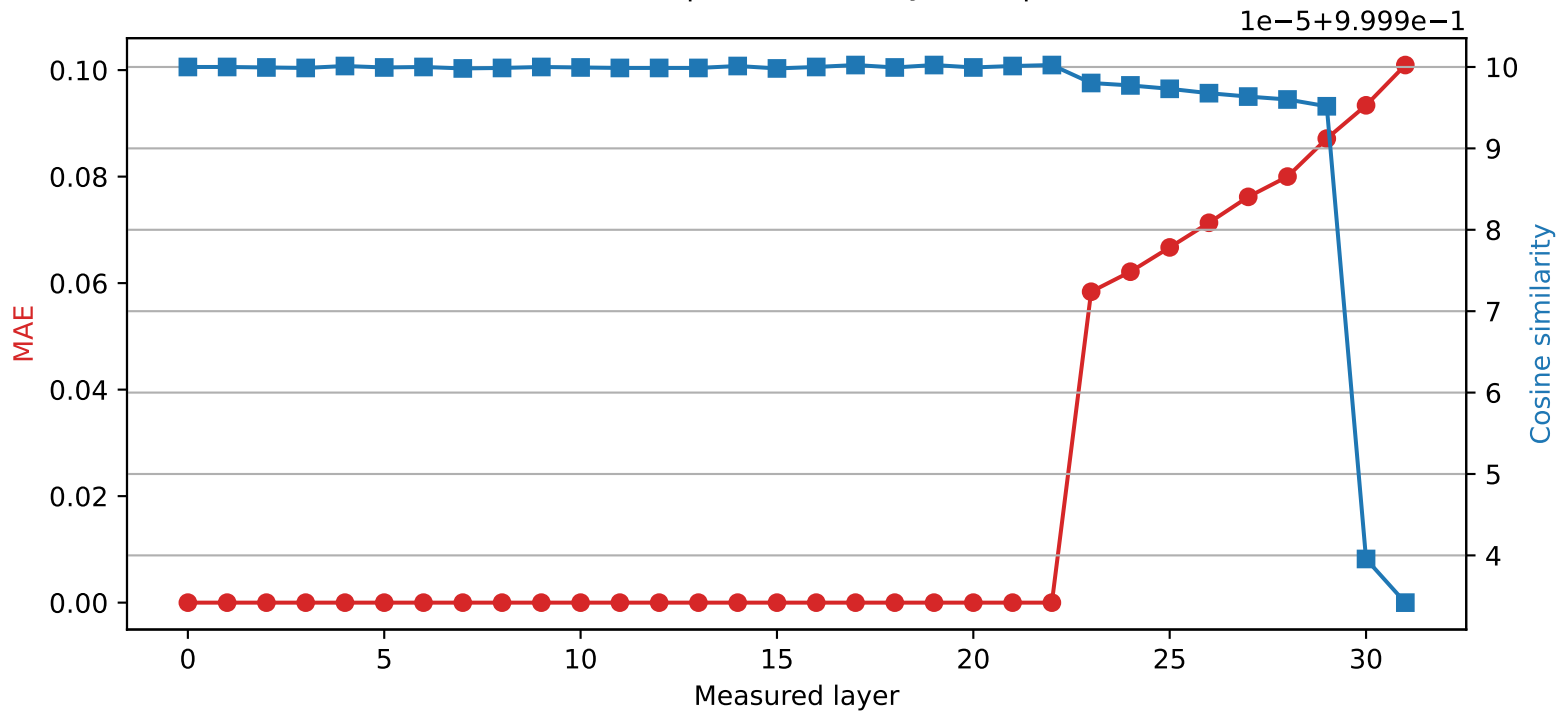
Phi-3-mini-4k-instruct | Quantized layer 22 | float32 \rightarrow int8
