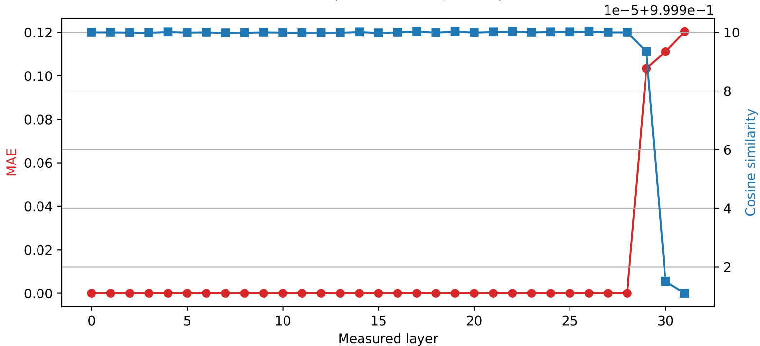
Phi-3-mini-4k-instruct | Quantized layer 28 | float32 \rightarrow int8
