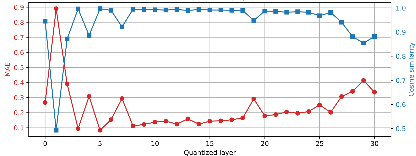
Phi-3-mini-4k-instruct | Prompt 0 Final RMSNorm output damage | float32 \rightarrow int4
