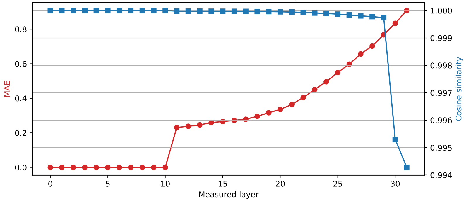
Phi-3-mini-4k-instruct | Quantized layer 10 | float32 \rightarrow int4
