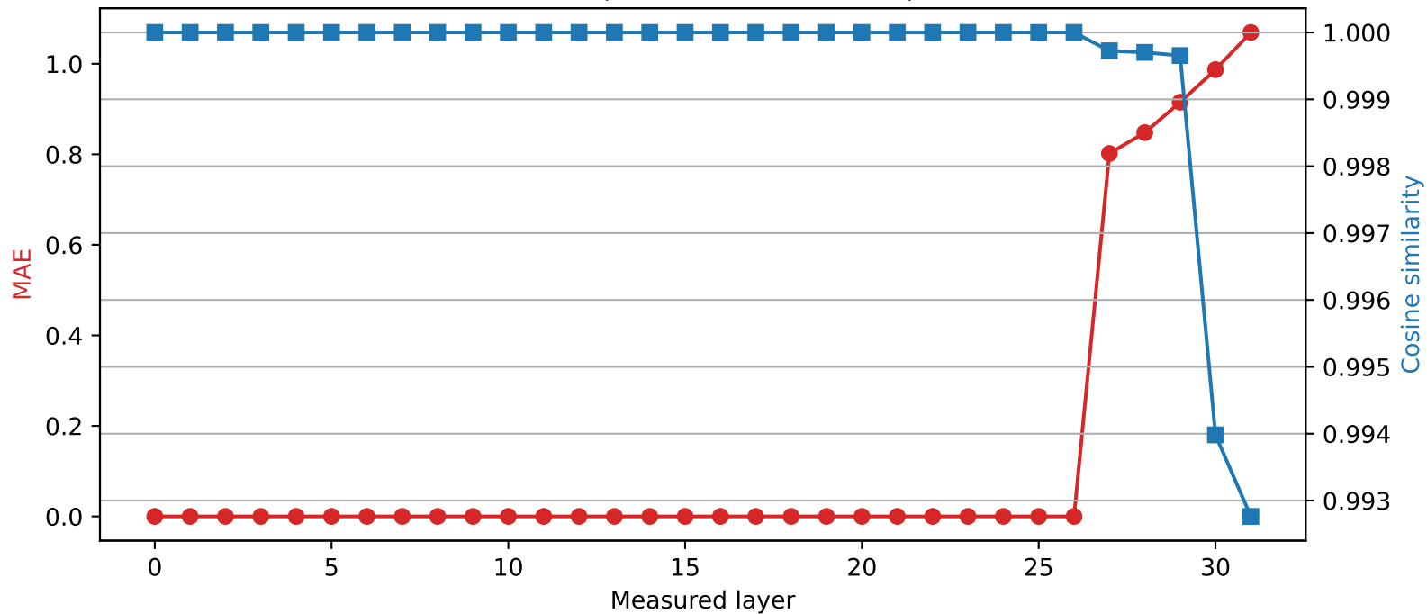
Phi-3-mini-4k-instruct | Quantized layer 26 | float32 \rightarrow int4
