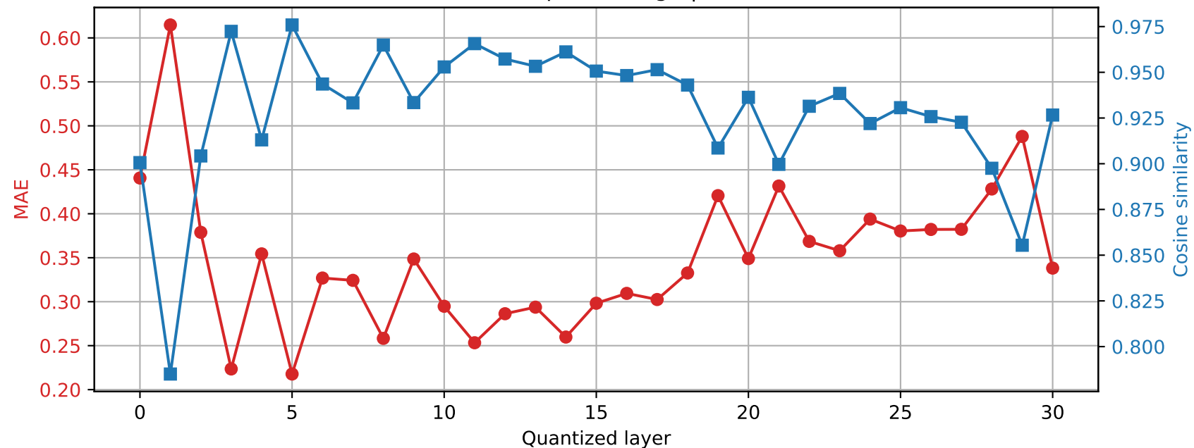
Phi-3-mini-4k-instruct | Prompt 1 Final RMSNorm output damage | float32 \rightarrow int4
