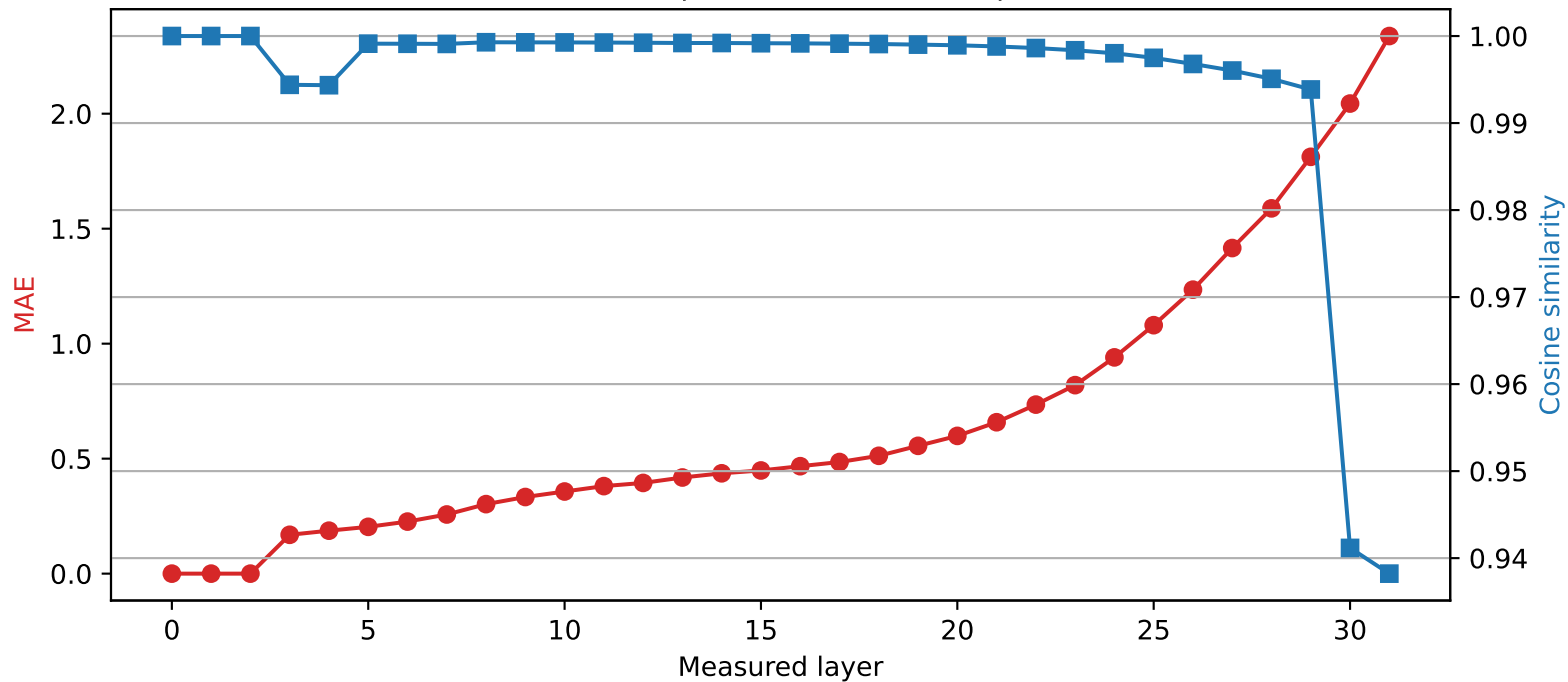
Phi-3-mini-4k-instruct | Quantized layer 2 | float32 \rightarrow int4
