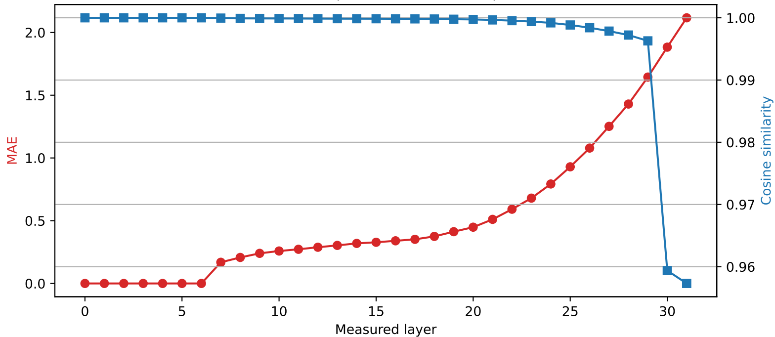
Phi-3-mini-4k-instruct | Quantized layer 6 | float32 \rightarrow int4
