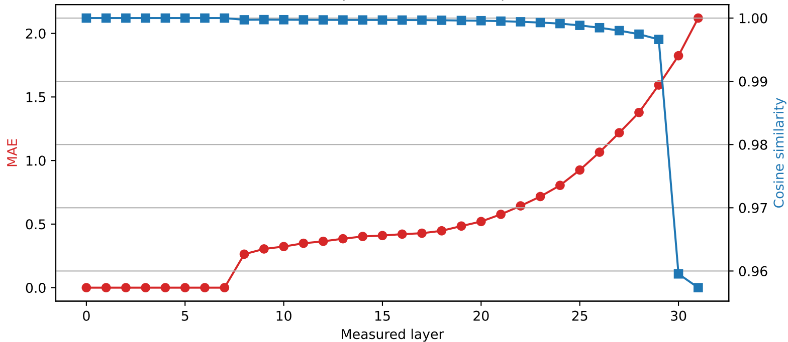
Phi-3-mini-4k-instruct | Quantized layer 7 | float32 \rightarrow int4
