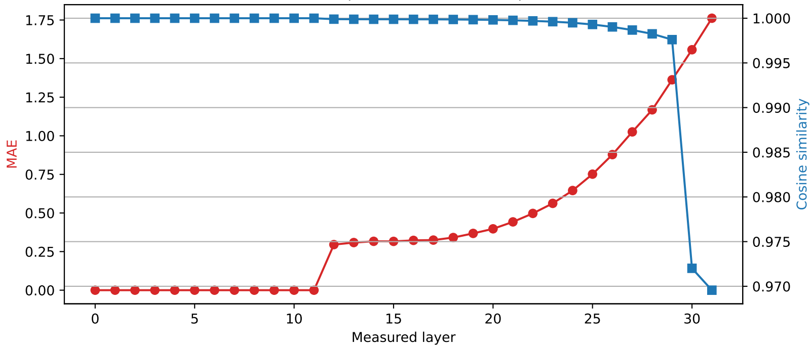
Phi-3-mini-4k-instruct | Quantized layer 11 | float32 \rightarrow int4
