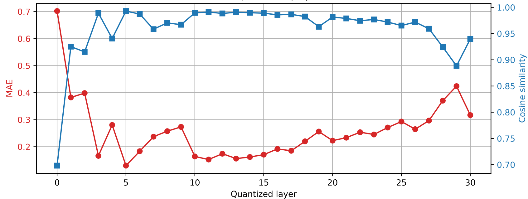
Phi-3-mini-4k-instruct | Prompt 2 Final RMSNorm output damage | float32 \rightarrow int4
