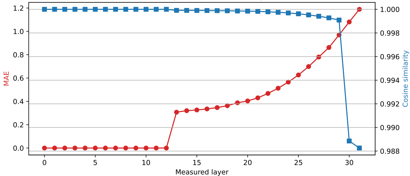
Phi-3-mini-4k-instruct | Quantized layer 12 | float32 \rightarrow int4
