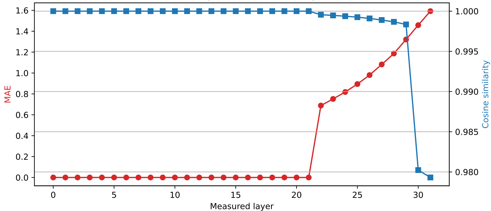
Phi-3-mini-4k-instruct | Quantized layer 21 | float32 \rightarrow int4
