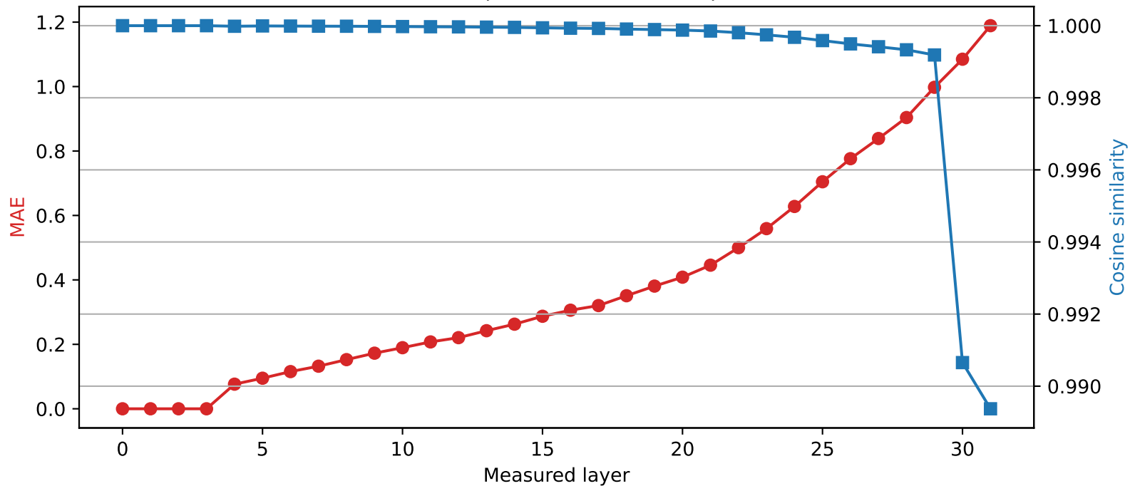
Phi-3-mini-4k-instruct | Quantized layer 3 | float32 \rightarrow int4
