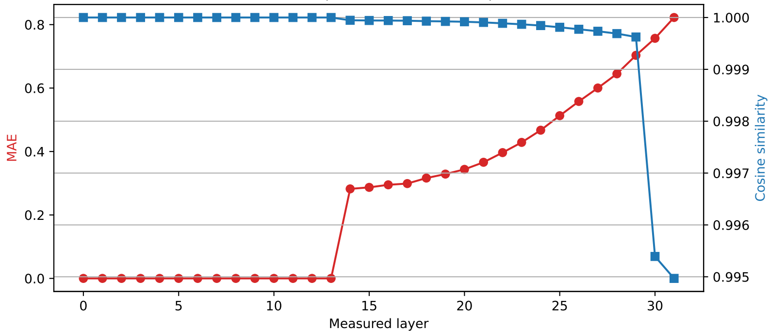
Phi-3-mini-4k-instruct | Quantized layer 13 | float32 \rightarrow int4
