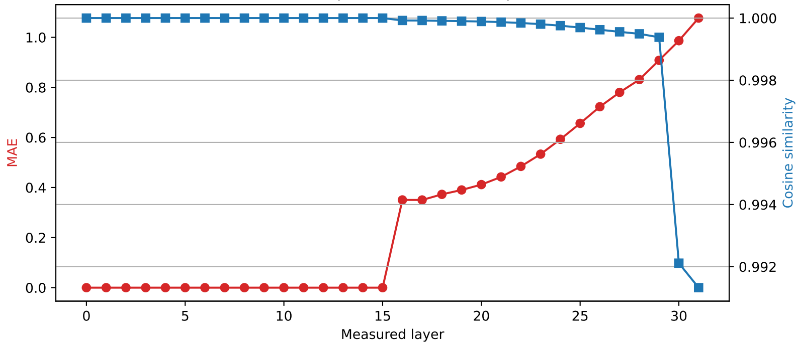
Phi-3-mini-4k-instruct | Quantized layer 15 | float32 \rightarrow int4
