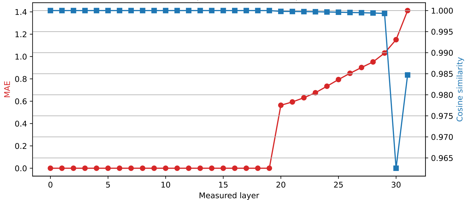
Phi-3-mini-4k-instruct | Quantized layer 19 | float32 \rightarrow int4
