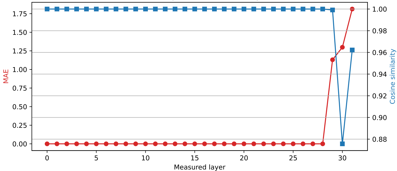
Phi-3-mini-4k-instruct | Quantized layer 28 | float32 \rightarrow int4
