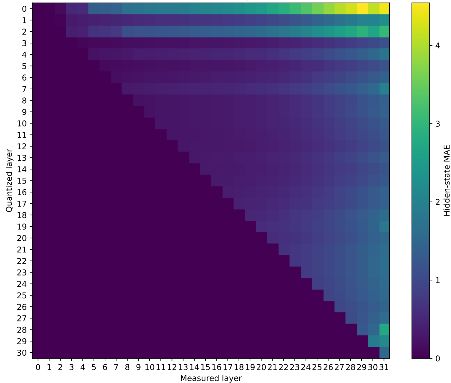
Model: Phi-3-mini-4k-instruct | float32 \rightarrow int2
