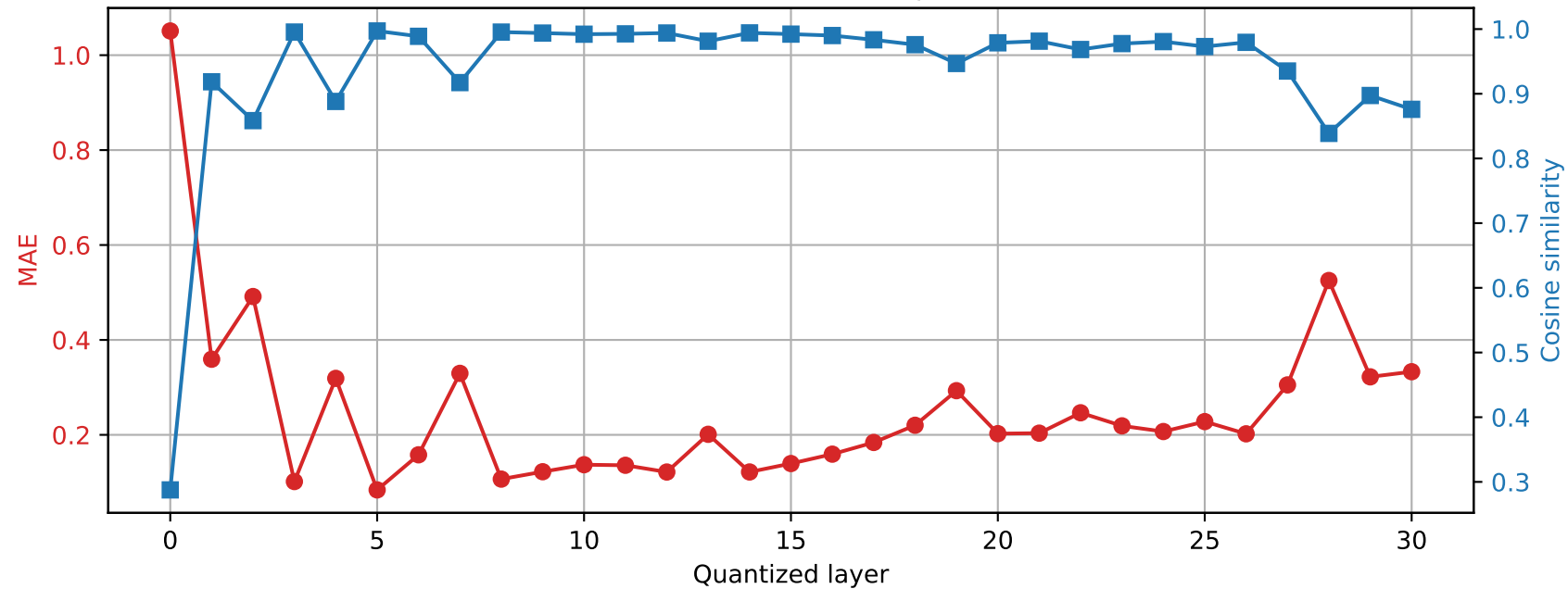
Phi-3-mini-4k-instruct | Prompt 0 Final RMSNorm output damage | float32 \rightarrow int2
